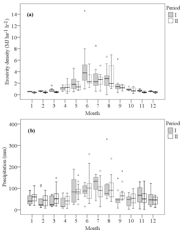
Figure 3. Monthly erosivity density (a) and monthly precipitation (b) for periods I and II. The bars with a dashed outline represent the growing seasons (April–October), the bars with a solid outline denote the dormant seasons (November–March), the whiskers indicate the range between the minimum and the maximum, and the asterisks indicate the outliers.
