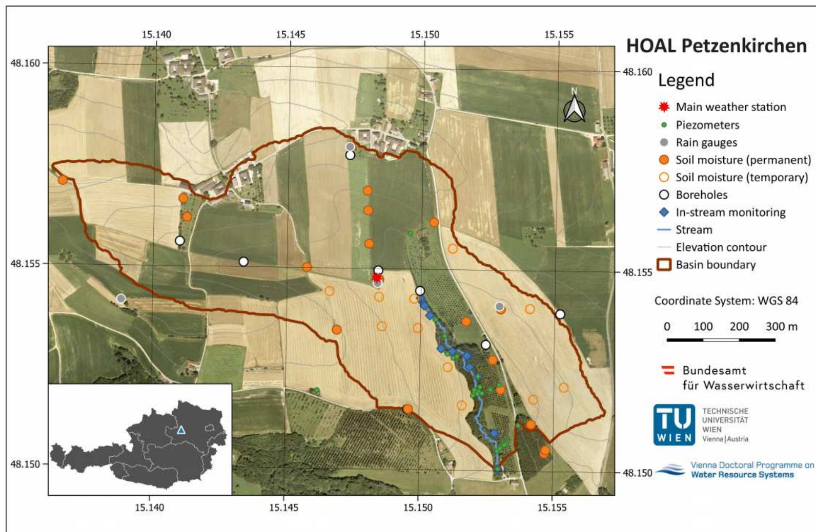
Figure 3. Overview of current equipment and measurements at HOAL Petzenkirchen, Austria.
